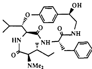
Pandamine ( 1 )
