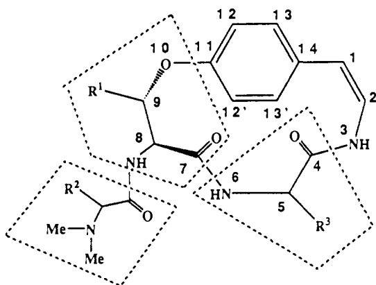
Figure 1. Structural features and numbering of a 14-membered cyclopeptide alkaloid.
